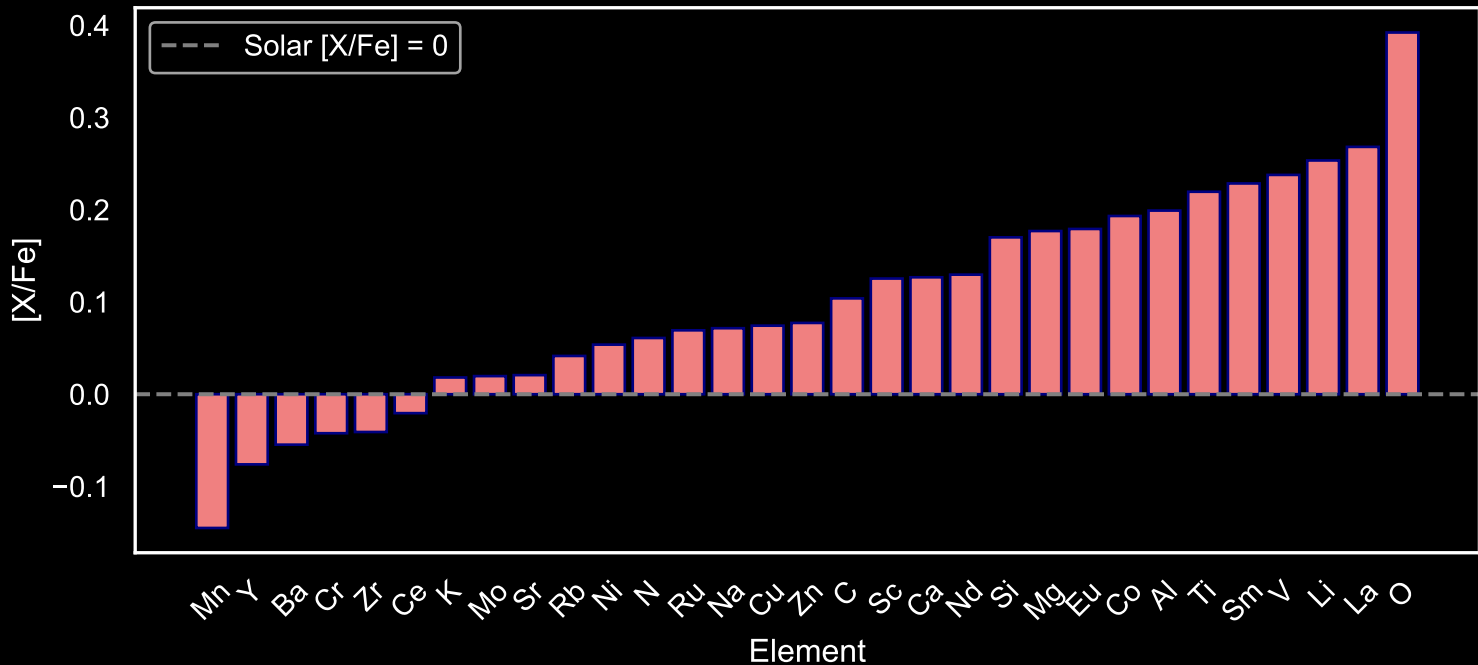
Abundance Pattern for GALAH Red Giants: Star Field [31] (N=52)
