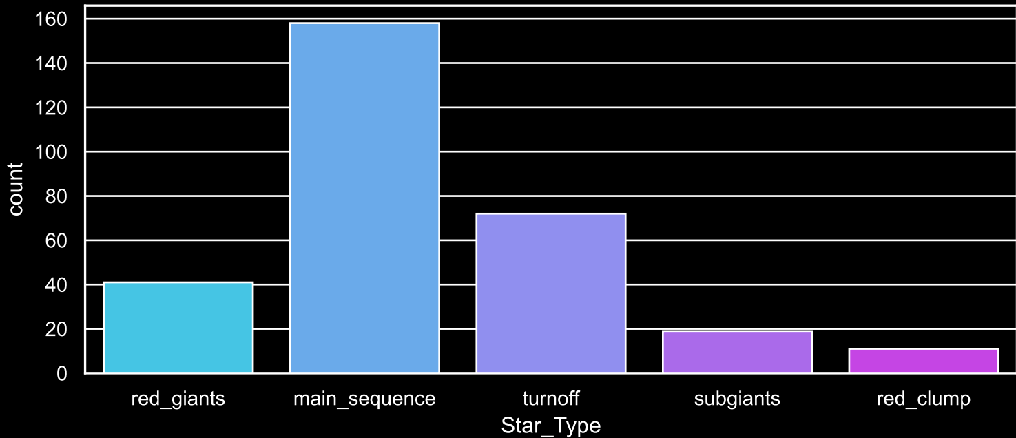
Field [31] Count plot of Star Type
