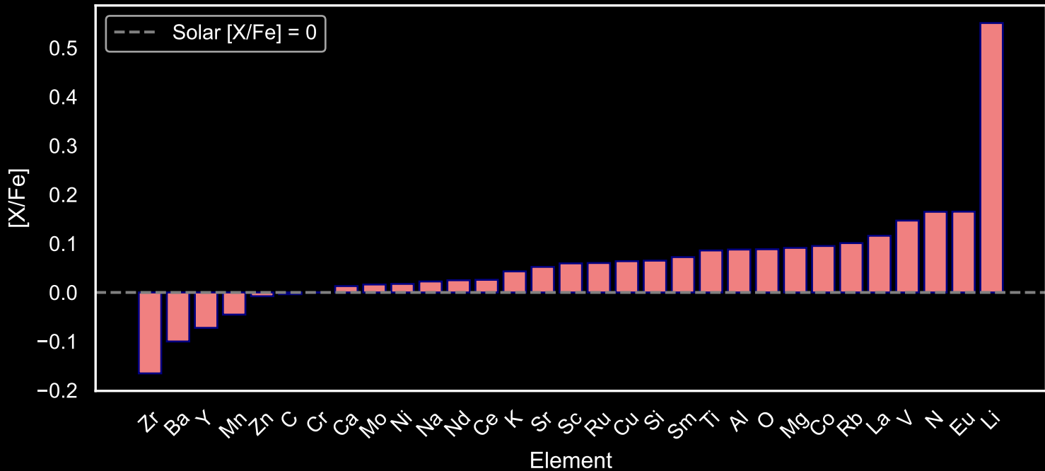
Abundance Pattern for GALAH Star Field [31] (N=301)
