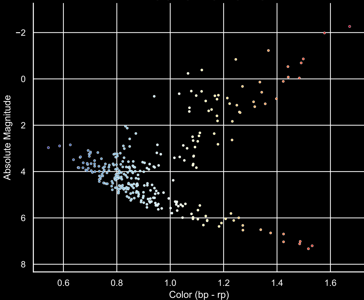
GALAH Hertzsprung-Russell Diagram Field [31] Ra [355.64] Dec [-69.74]
