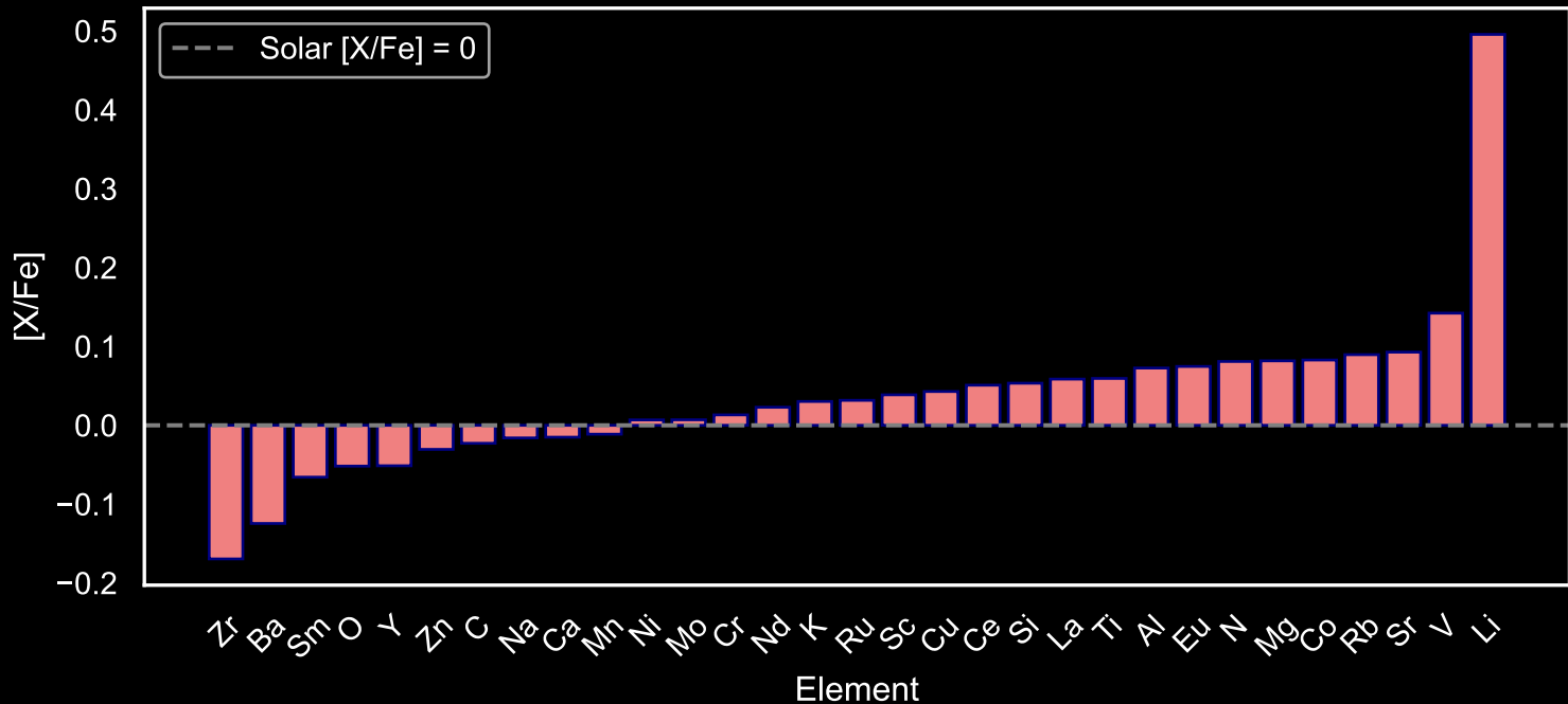
Abundance Pattern for GALAH Main Sequence Stars: Star Field [31] (N=158)
